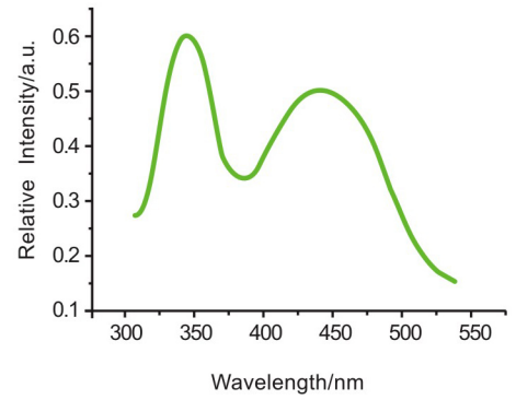
激发光谱 EX Spectrum
